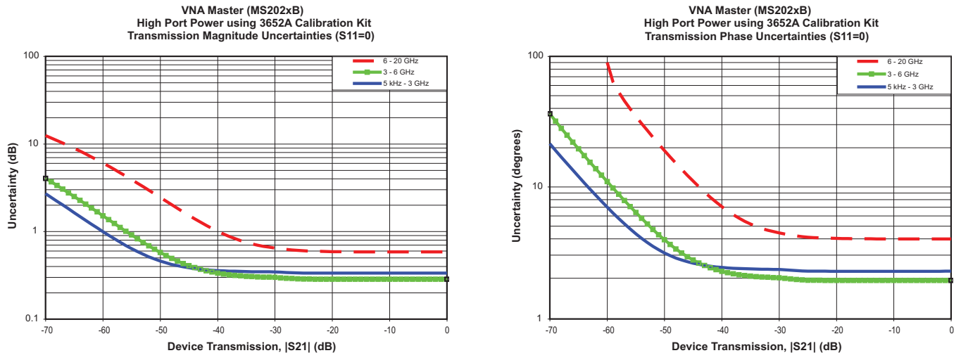
These two transmission uncertainty curves, magnitude on the left and phase on the right, describe the MS202xB's worst-case uncertainties for S_{21} transmission measurements when using the high port power setting. Each trace represents the frequency range described in the legend. The transmission magnitude uncertainties for S_{21} measurements between 0 and 30 dB is less than 0.6 dB. Similarly, the transmission phase uncertainties for S_{21} measurements between 0 and 30 dB is less than 4°. The typical uncertainties are nearly 10x better than scalar based transmission measurements.
