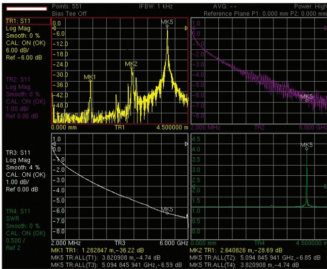
The VNA Master has a flexible display that can simultaneously view S_{11} , as distance-to-fault (log magnitude), return loss, cable loss with smoothing (Log Mag |S_{11}| / 2), and distance-to-fault (SWR). On the left is a four trace display in quad format. On the right is a two trace display in single overlay format. A single keystroke toggle can maximize and minimize individual traces for additional viewing flexibility.
