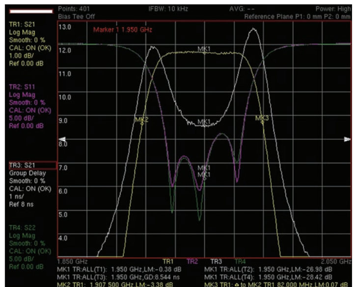
A two-port filter measurement is shown using a four trace overlay feature. This measurement reveals that the filter is well matched, the passband flatness is acceptable, and the group delay is within specification. A portable tool with fast sweeps of 750 \mu sec/point can even offer real-time tuning of this device on site.
